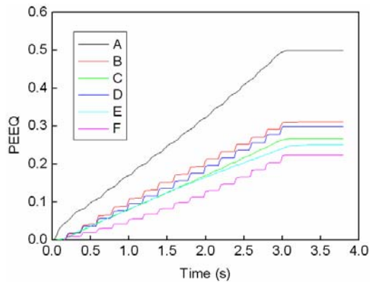
(b) PEEQ history of tracking points in cold rotary forging
