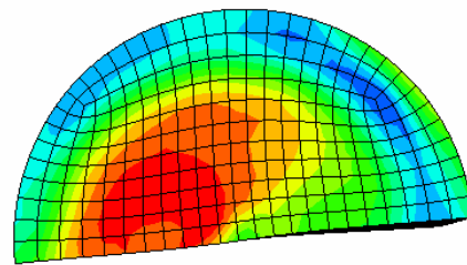
(c) After deformation in cold rotary forging
